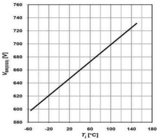
Typ.Drain-source breakdown voltage
