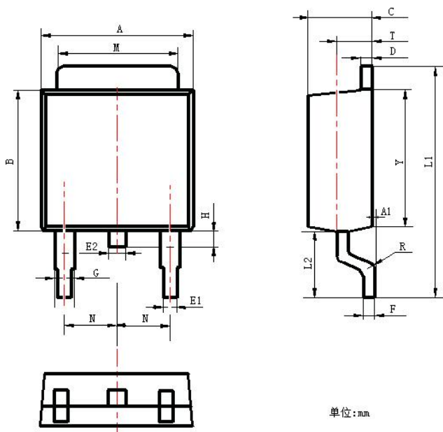
TO-252-2L
