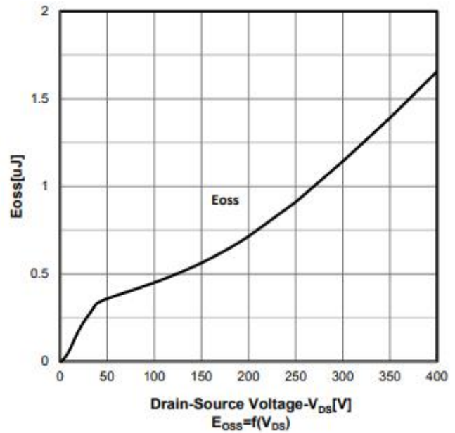
Typ.Coss stored energy
