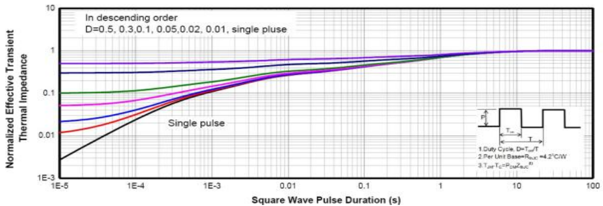
Max. transient thermal impedance TO-220F
